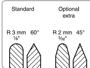
Exchangeable discs. Full scale.
